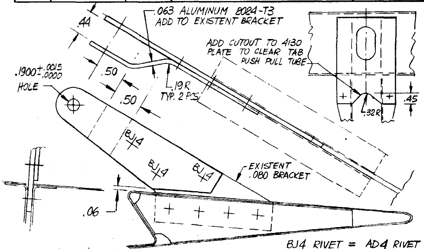
DWG 1-20-003 - STABILATOR
